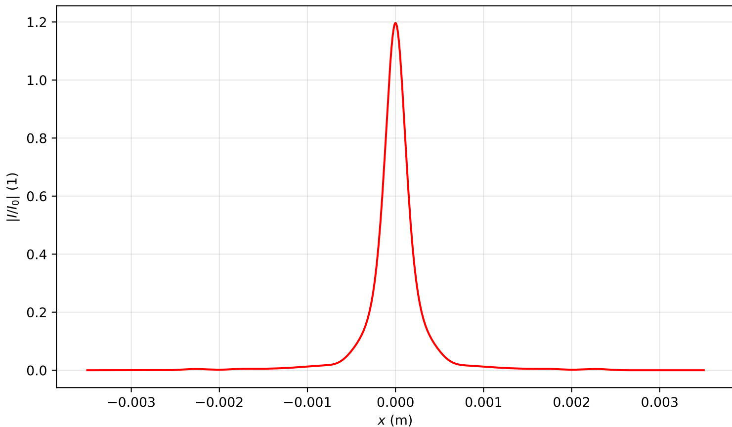
Intensity profile I(x, y = 0, z = 3.821)/I_0 , \text{Pin}=3.0\text{Pcr} , artificial time
